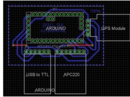
Figure 8 Desain PCB Board
