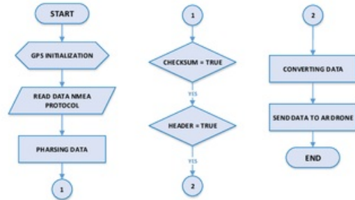
Figure 5 Microcontroller Programming flowchart
