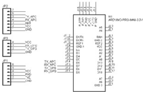
Figure 7 Schematic Design
