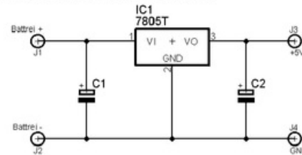
Figure 9 Regulator Schematic
