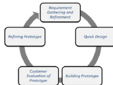
Gambar 3. Metode prototype
