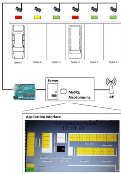
Figure-2. Schematic diagram.
