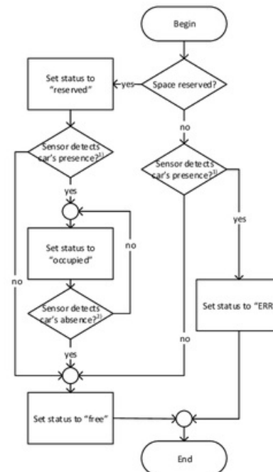
Figure-6. Parking status flowchart.
